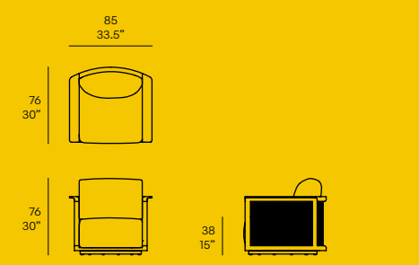
[OTANUA05] NUANCE SWIVEL CLUB CHAIR
